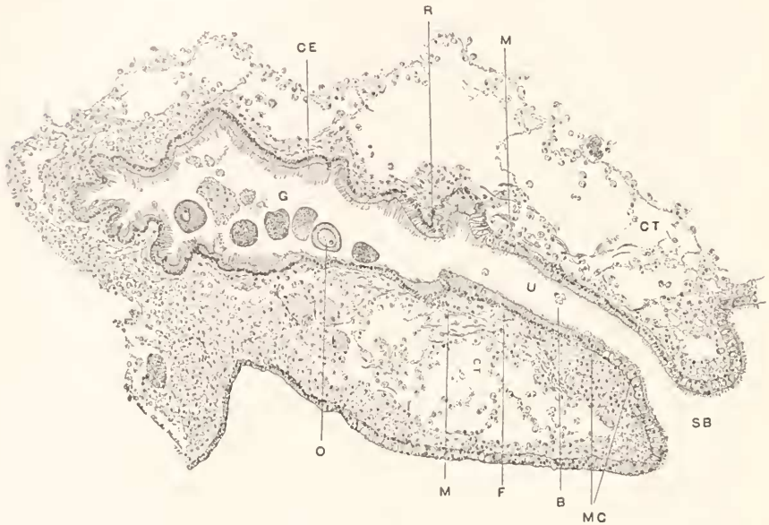
FIG. 2. Ostrea edulis , transverse section of the right urinogenital cleft and oviduct preserved during ovulation. Camera lucida drawing \times 150 . Hæmateïn-cosin.
